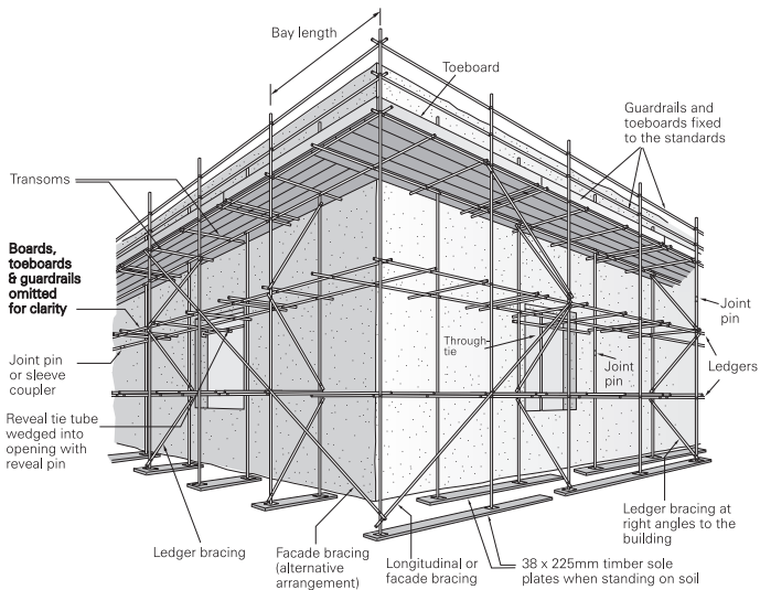
Typical independent tied scaffold
